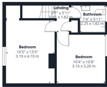
Floor 1
